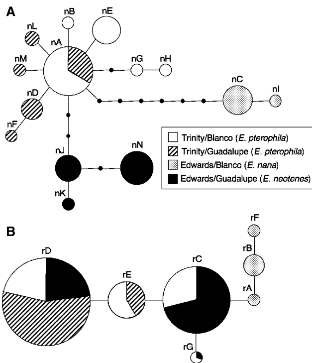
Fig. 2 Maximum parsimony network for ND4 (mtDNA; A) and rag1 (nuclear DNA; B). A circle represents each haplotype and the size of each circle is approximately proportional to the frequency of the haplotypes in the dataset. Haplotypes are marked as clear (Trinity Aquifer/Blanco River system, E. pterophila ), striped (Trinity Aquifer/Guadalupe River system, E. pterophila ), dotted (Edwards Aquifer/Blanco River system, E. nana ), and solid (Edwards Aquifer/Guadalupe River system, E. neotenes ) according to the proportion of individuals that belong to springs on the respective aquifer and river system
